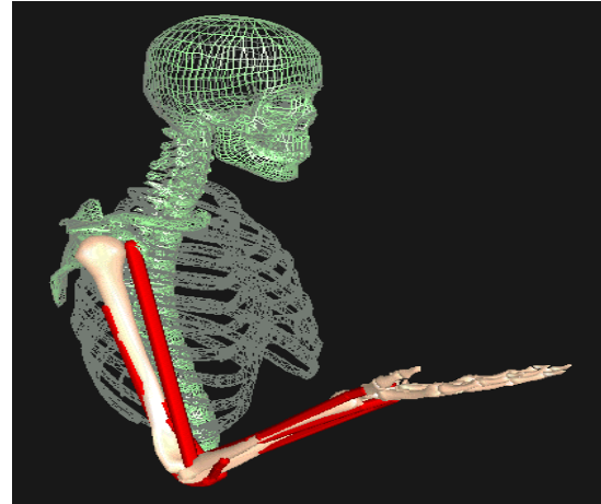
Figure 2. The anatomical model of the arm in SIMM
